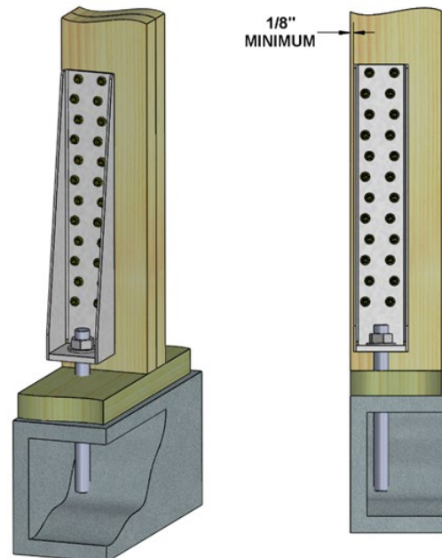
TYPICAL UPHD INSTALLATION
