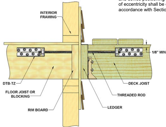
TYPICAL DTB-TZ INSTALLATION
