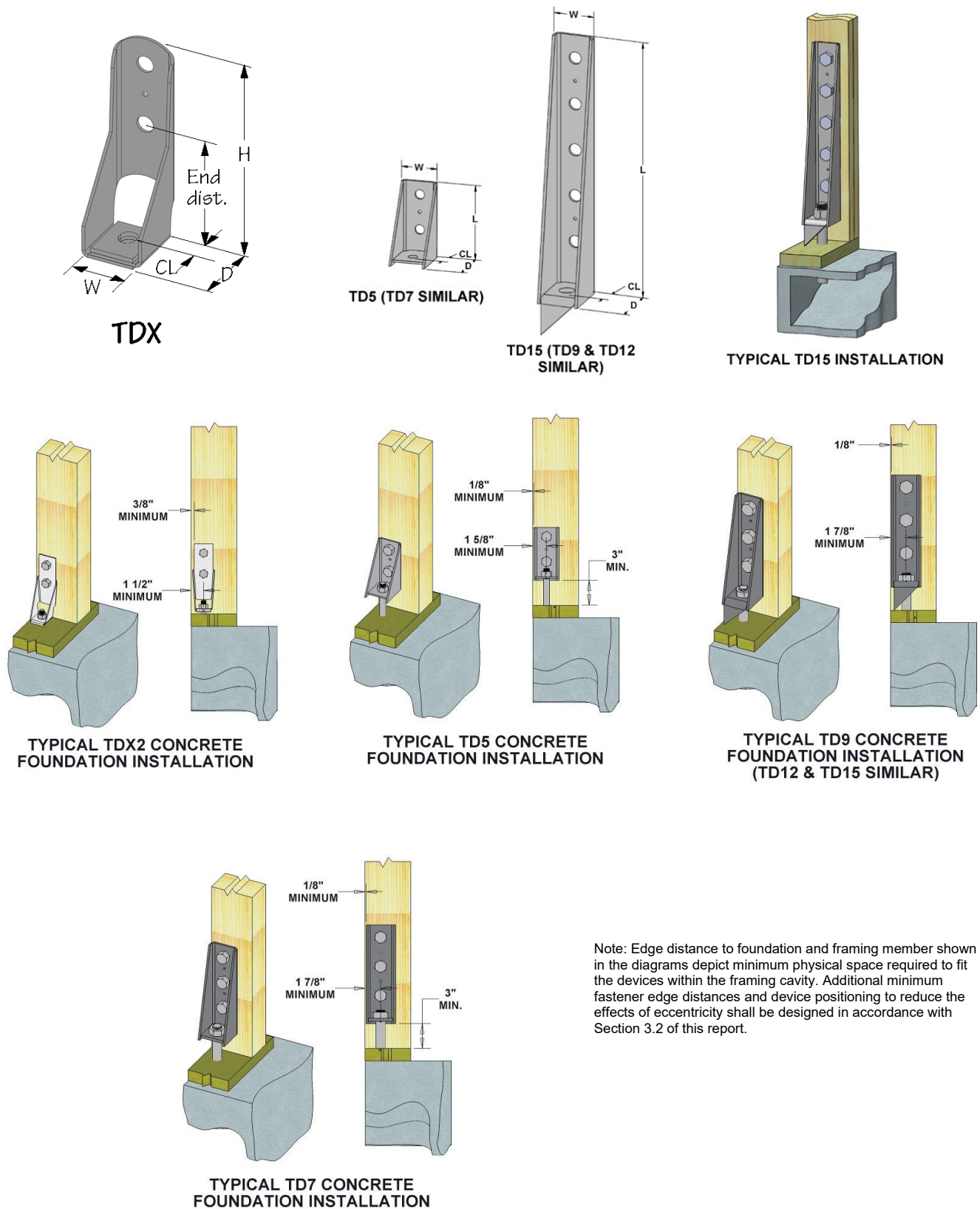
FIGURE 3 – TD AND TDX HOLD-DOWNS
