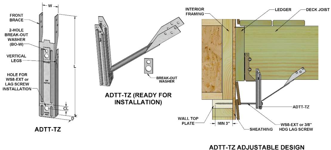
FIGURE 7 – ADTT-TZ CONNECTOR
