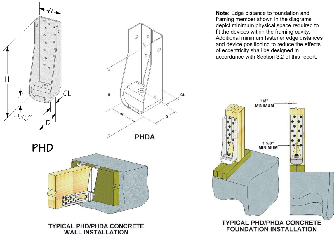
FIGURE 1 – PHD AND PHDA HOLD-DOWNS
