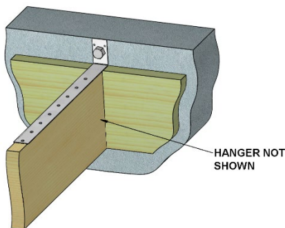
TYPICAL TS19-TZ INSTALLATION (LTS20B & LTTI31 SIMILAR)
