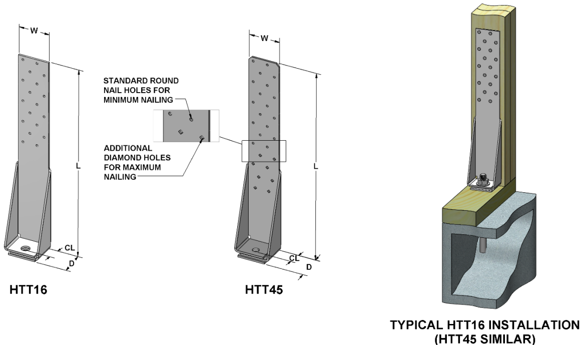
FIGURE 4 - HTT TENSION TIE HOLD-DOWNS
